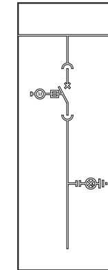
Kublay Hücresi Coupling Switchgear
